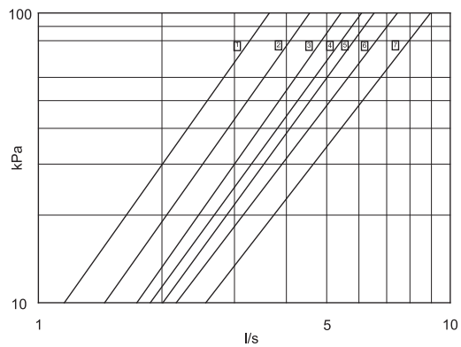
Figure 5 - Condenser water pressure drop
