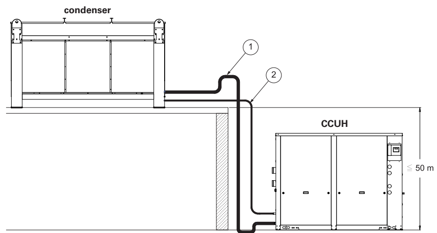
Figure 2 - Installation configuration - CCUH below condenser
