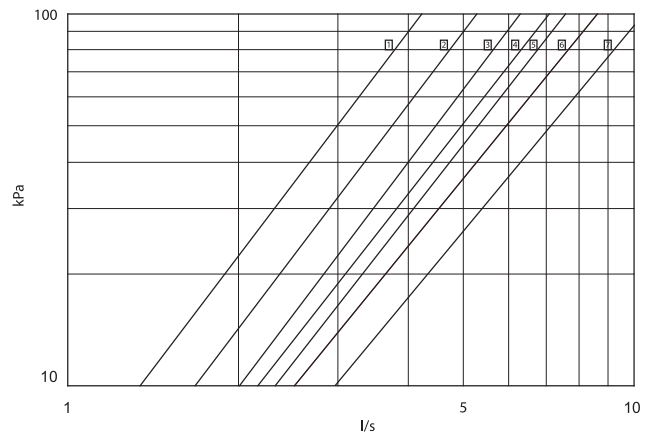
Figure 4 - Evaporator water pressure drop
